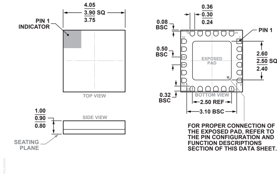
24-Terminal Ceramic Leadless Chip Carrier [LCC] (E-24-1)
